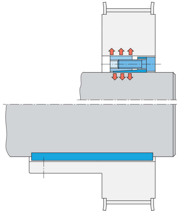
Upper half of figure: Shaft-hub-connection with Cone Clamping Element
