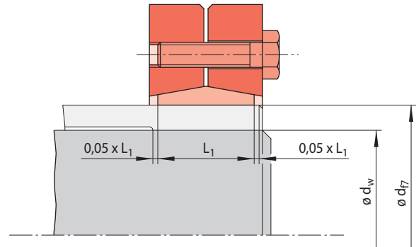
Shrink Disc clamped
