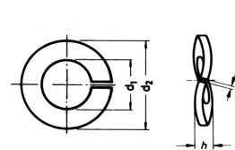
Form B
